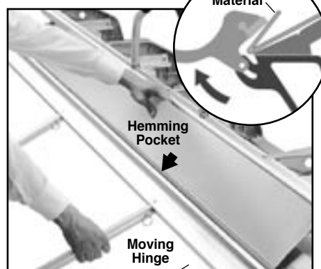
5 Position the bent edge of the material in the Hemming Pocket on top of the Anvil.
