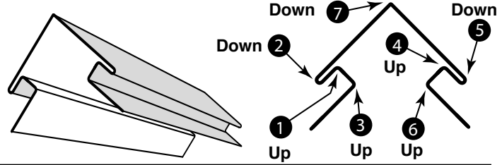
7. Counter Flashing
